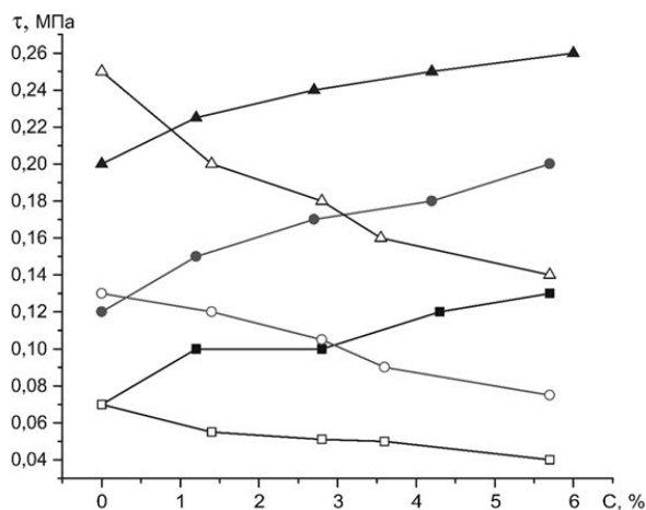
Fig. 4. Dependences of the strength of saline clay soils: 0.1 MPa (■); 0.2 MPa (●); 0.3 MPa (▲); natural moisture content – flooded symbols; water saturation – not flooded symbols
