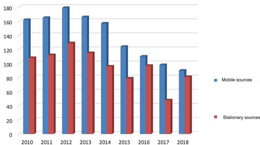
Fig. 2. Dynamics of pollutant emissions from mobile and stationary sources of Kyiv region in 2010-2018
